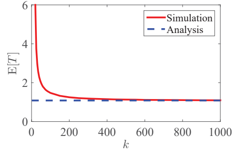
Fig. 4. Mean response time under RIQ from analysis (dashed blue line) and simulation (solid red line, 99% confidence intervals are within the line) when \lambda = 0.7 , d = 20 , X \sim \text{H2} with \mathbf{E}[X] = \frac{1}{4.7} and C_X^2 = 10 , and S \sim \text{Dolly}(1, 12) . When k = 1000 , the analysis is within 1% of simulation.
