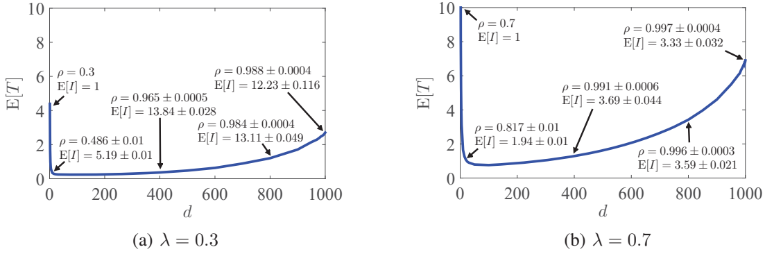
Fig. 8. Mean response time under RIQ (simulated) as a function of d when k = 1000 , X \sim H2 with \mathbf{E}[X] = \frac{1}{4.7} and C_X^2 = 10 , S \sim \text{Dolly}(1, 12) , and (a) \lambda = 0.3 , (b) \lambda = 0.7 . While mean response time increases as d gets close to k , even when d = k mean response time is lower than when d = 1 . The lines are annotated with the values of \rho and \mathbf{E}[I] (the expected number of copies per job) at several different values of d . 99% confidence intervals are within the line for \mathbf{E}[T] and are explicitly shown for \rho and \mathbf{E}[I] .
