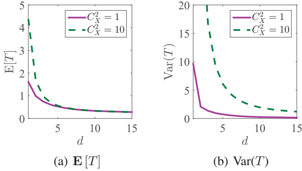
Fig. 7. (a) Mean, and (b) Variance of response time, T , (via analysis) under RIQ when \lambda = 0.3 , X \sim H2 with \mathbf{E}[X] = \frac{1}{4.7} and C_X^2 = 1 and 10, and S \sim \text{Dolly}(1, 12) . As d increases, both the mean and the variance of response time decrease; the improvement is more pronounced in the variance.
