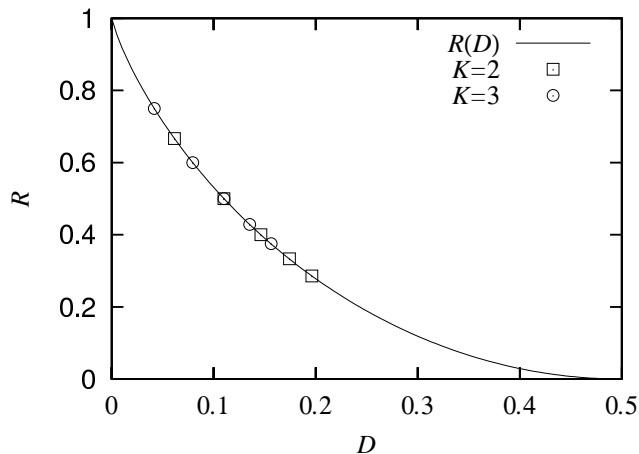
Figure 2: Numerically-constructed stable solutions: Stable solutions of (15) for the finite values of K and L are calculated by using Monte Carlo methods. We use 10^5 bin models to approximate the probability distributions \pi_{\text{IRSB}}(x) and \hat{\pi}_{\text{IRSB}}(\hat{x}) , starting from various initial conditions. The distributions converge to the \delta peaks, giving almost optimal performance. ( \square ) K = 2 and L = 3, 4, \dots, 7 ; ( \circ ) K = 3 and L = 4, 5, \dots, 8 ; Solid line indicates the rate distortion function R(D) .
