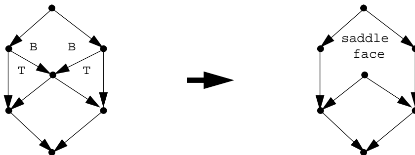
Figure 16: Example of intra-rule conflict for TB Rule
