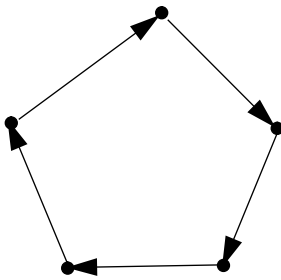
cycle face
