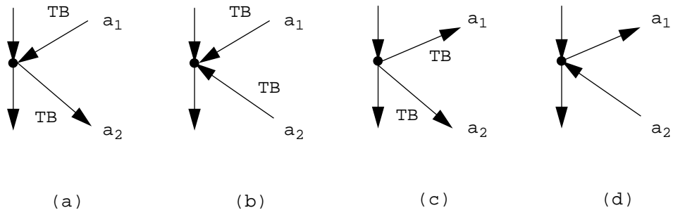
Figure 21: Consecutive Type II TB Arc Incidences at a Vertex
