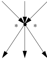
flow vertex
