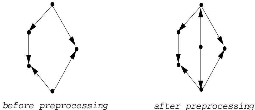
Figure 4: Preprocessing Saddle Faces
