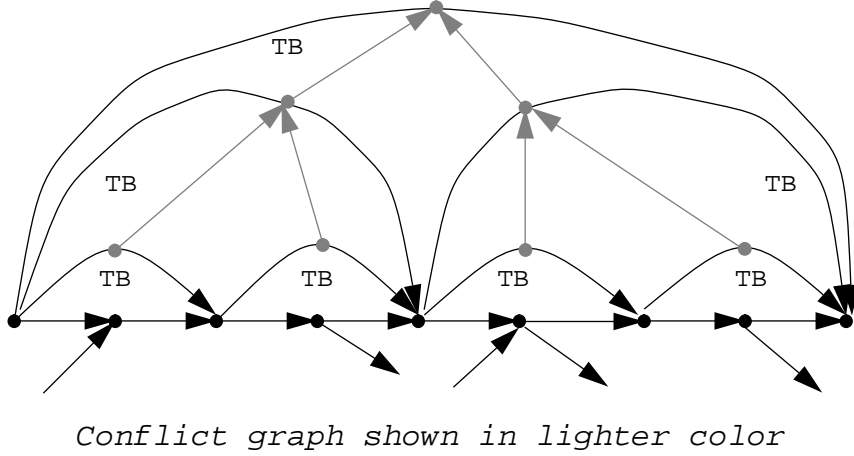
Figure 20: Conflict Graph for First Phase of Type II TB Conflict Resolution
