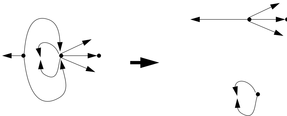
Figure 12: Index 1 Saddle Rule – Single Degree-3 Source Case
