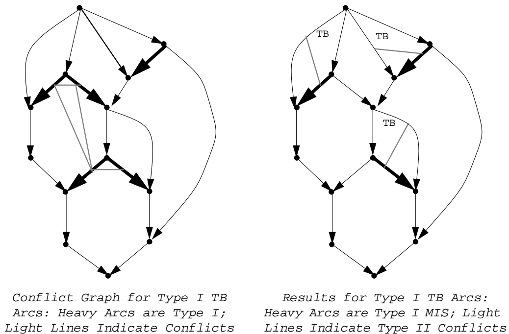
Figure 18: TB Rule Conflict Graphs
