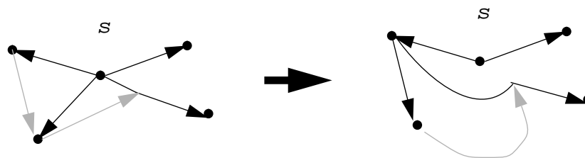
Figure 13: Cleanup: Realignment at a Source
