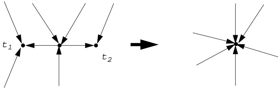
Figure 11: Index 1 Saddle Rule Applied to Sinks – both arcs contracted
