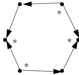
saddle face
