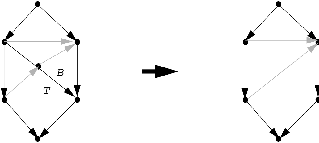
Figure 5: TB Rule Pointer Splicing
