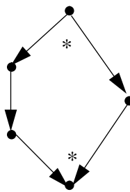
flow face
