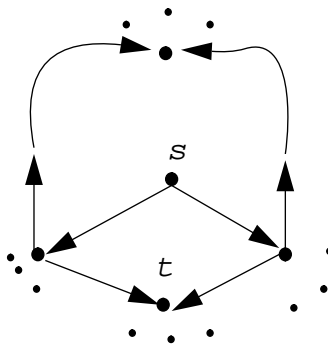
Figure 14: Degree-2 source with common adjacent eligible sink
