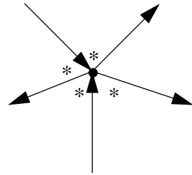
saddle vertex
