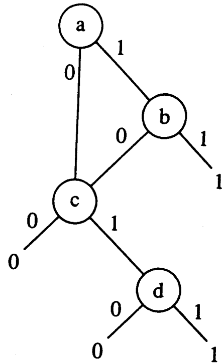
Fig. 1. A binary decision diagram.
