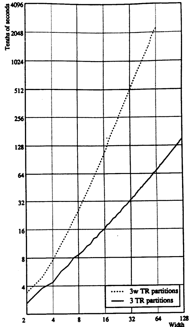
Fig. 6. Verification times for MINMAX circuit.
