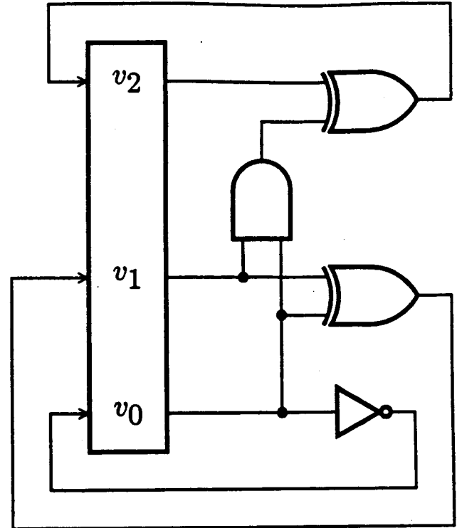
Fig. 2. Synchronous modulo 8 counter.
