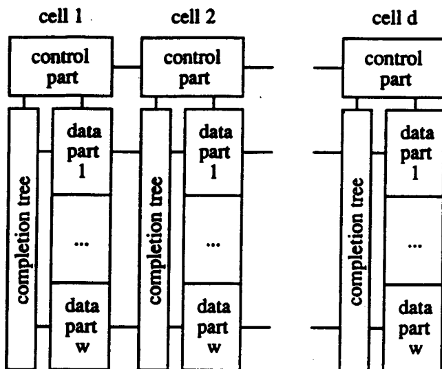
Fig. 8. Stack circuit block diagram.
