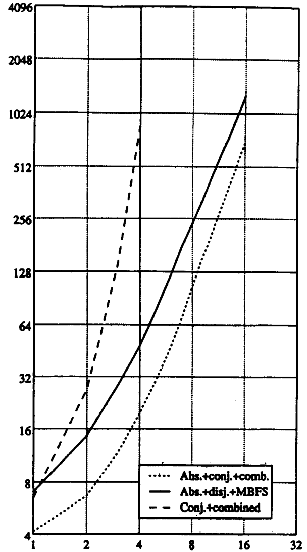
Fig. 10. Search times in seconds for stacks of various depths, with w = 1 .
