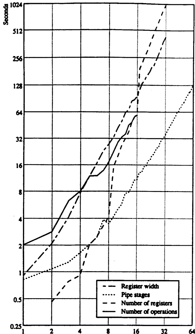
Fig. 5. Pipeline circuit verification times.
