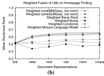
Figure 3: Results for Homepage Finding. The fusion algorithms are weighted. (a) Okapi (b) language models
