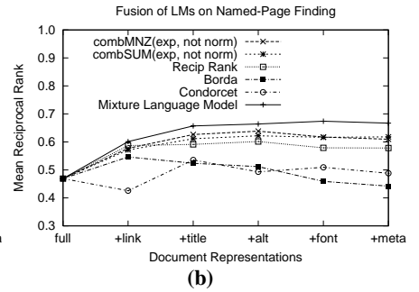
Figure 4: Results for Named-Page Finding. The fusion algorithms are unweighted. (a) Okapi (b) language models
