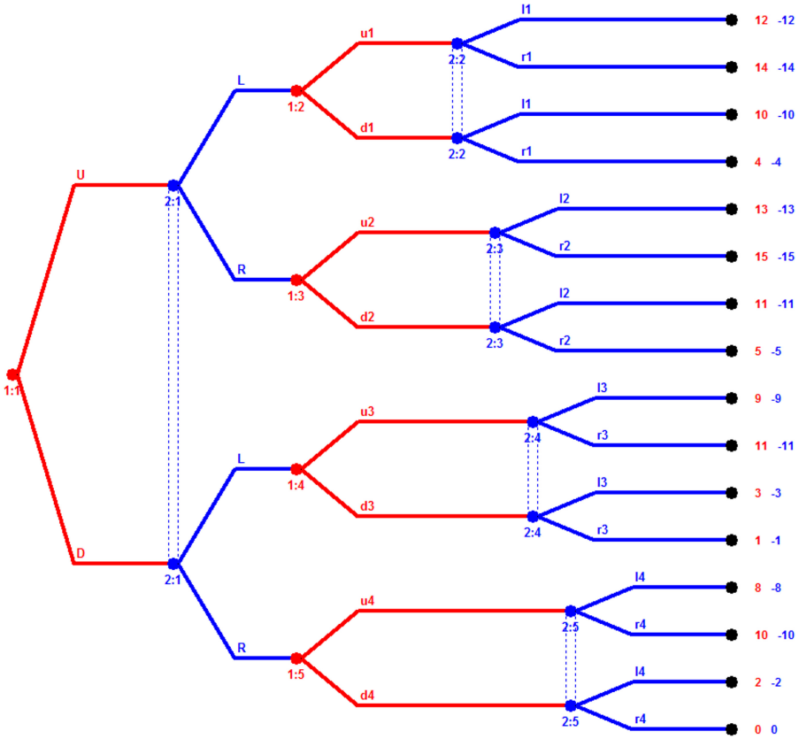
Fig. 9. Extensive-form representation of a game where we can detect and exploit a gift within a game iteration. X:Y denotes the Y th information set of Player X . Dotted lines tie together nodes within an information set. At leaves of the game tree, the payoff of Player 1 is listed first, followed by the payoff of Player 2.
