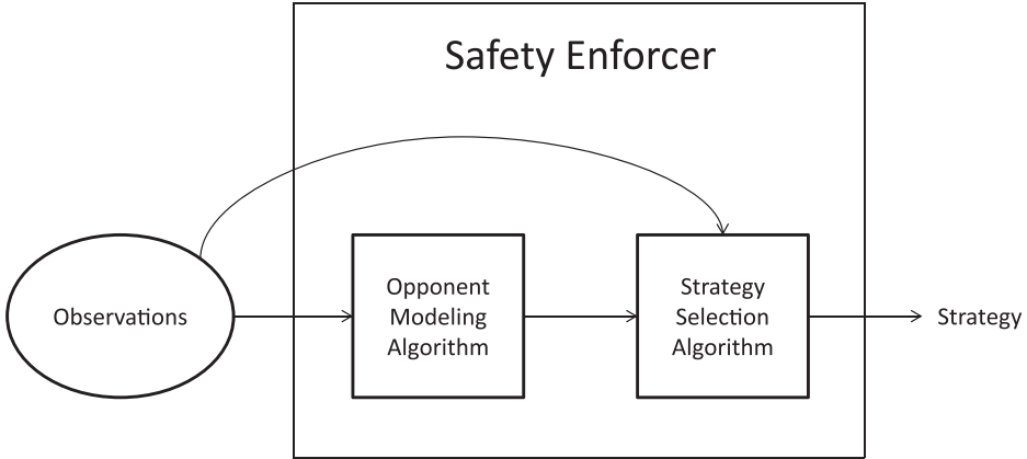
Fig. 1. Our safe exploitation methodology used as a meta-algorithm which makes any opponent exploitation architecture safe. An opponent exploitation architecture consists of two components: an opponent modeling algorithm and a strategy selection algorithm.
