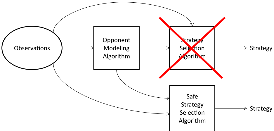
Fig. 2. Our safe exploitation methodology used to replace the strategy selection component while retaining the opponent modeling component of any opponent exploitation architecture.
