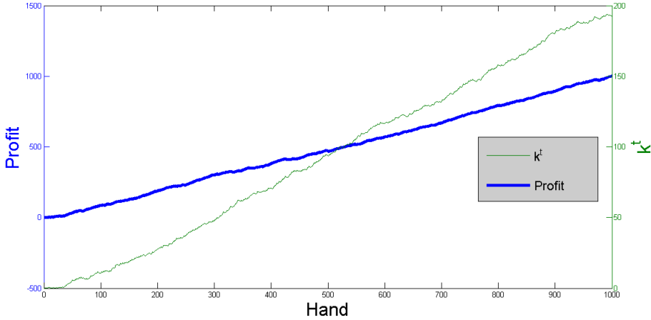
Fig. 10. Profit and k^t over the course of a match of RWYWE against a random opponent. Profits are denoted by the thick blue line using the left Y axis, while k^t is denoted by the thin green line and the right Y axis. Against this opponent, both k^t and profits steadily increase.
