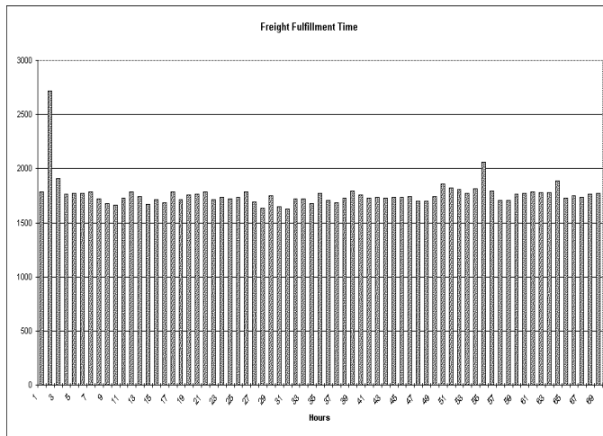
Fig. 15. The average time for task performance (y axis) in the case of agents and tasks normally distributed around the center of the city. The execution time decreased significantly compared to an even distribution (except for the first hour of the simulation).
